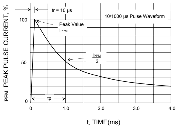
FIG.1 - PULSE WAVEFORM
